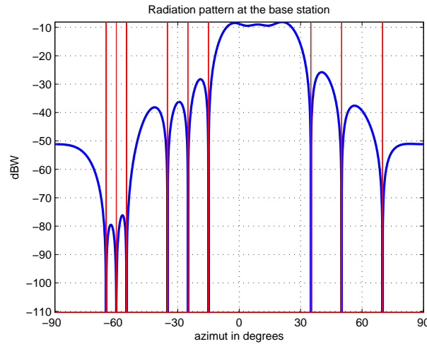
Figure 3: Radiation pattern of the base station, for the problem with three SINR constraints and nine null-shaping interference constraints and K = 12 . The required transmit power is 15.95 dBm.
