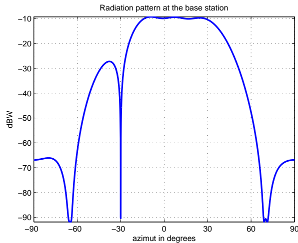
Figure 4: Radiation pattern of the base station, for the problem with three SINR constraints, one null interference constraint, two robust null interference constraint, and K = 8 . The required transmit power is 16.94 dBm.
