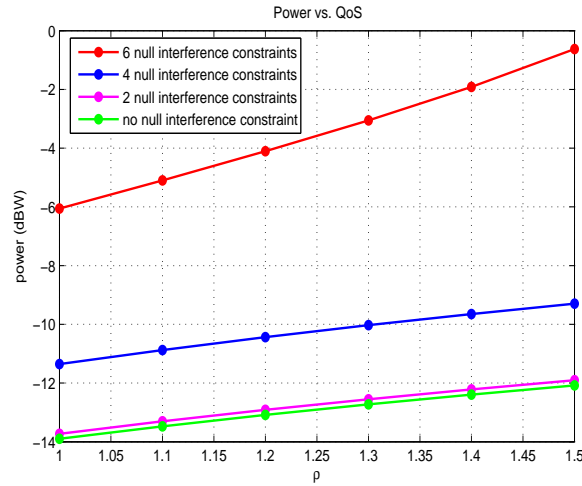
Figure 2: Minimal transmission power versus the threshold of SINR, with different numbers of null interference constraint.
