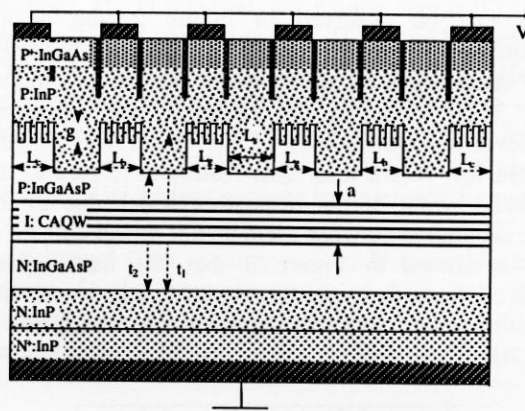
Figure 1. Longitudinal cross-section of the filter.
