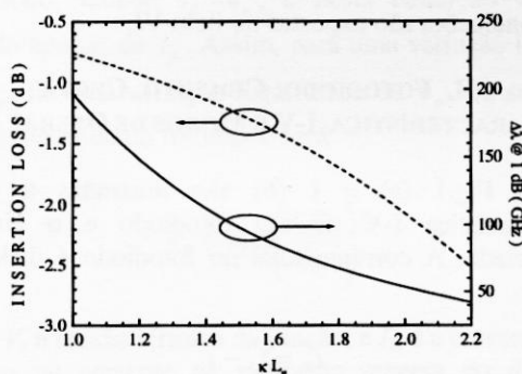
Figure 4. Insertion loss and bandwidth as a function of KL_g .
