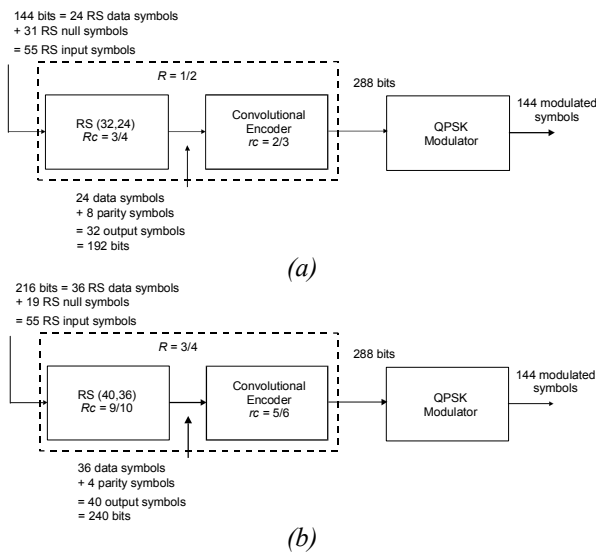
Figure 8 - Serial concatenation of Reed-Solomon with convolutional code: coding parameters for QPSK modulation with (a) code rate = 1/2; (b) code rate = 3/4.
